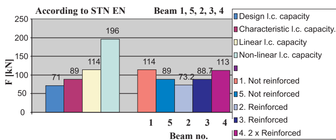
Fig. 12: Comparison of theoretically and experimentally researched load-carrying capacities
