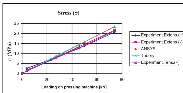
Fig. 11: Comparison of beam №5 stresses
