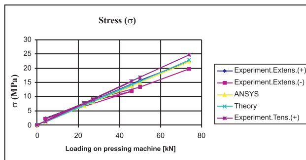
Fig. 9: Comparison of beam №3 stresses
