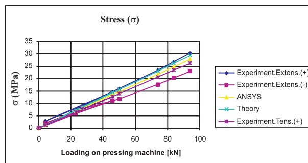
Fig. 10: Comparison of beam №4 stresses
