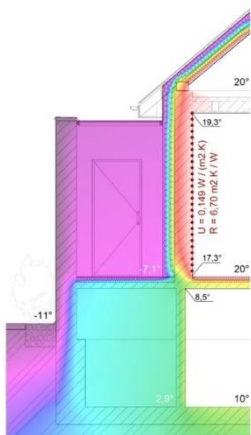
Variant C Transparent roof, non-transparent vertical constructions
