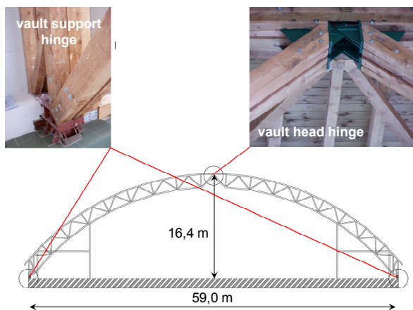
Figure 4 Three-hinged arch
